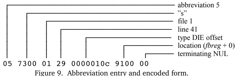
Figure 9. Abbreviation entry and encoded form.
